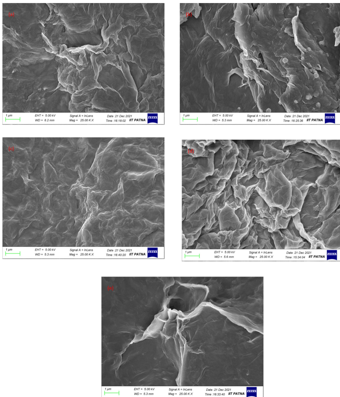
Fig. 15 FE-SEM images of GO in the presence of NaFlu (a) in neat water, (b) in a water–ACN ( \chi_{\text{ACN}} = 0.062 ) binary mixture, (c) in a water–DMF ( \chi_{\text{DMF}} = 0.080 ) binary mixture, (d) in a water–DMSO ( \chi_{\text{DMSO}} = 0.060 ) binary mixture and (e) in a water–THF ( \chi_{\text{THF}} = 0.022 ) binary mixture. \chi is the mole fraction of the co-solvent.
