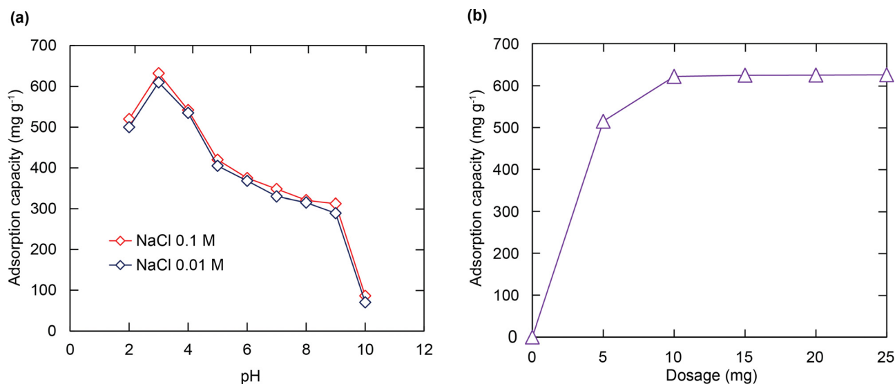
Fig. 4 Influence of solution pH value and ionic strength on the adsorption capacity of RhB over \text{H}^+ \text{c} \text{BUT-8(Cr)} [ m = 10 \text{ mg} , C_0 = 200 \text{ mg L}^{-1} , V_{\text{RhB}} = 50 \text{ mL} , t = 24 \text{ h} ] (a); Effect of \text{H}^+ \text{c} \text{BUT-8(Cr)} content on the RhB adsorption uptake [ m: 5\text{--}25 \text{ mg} , C_0 = 200 \text{ mg L}^{-1} , V_{\text{RhB}} = 100 \text{ mL} , \text{pH} = 3 , t = 24 \text{ h} ] (b).
