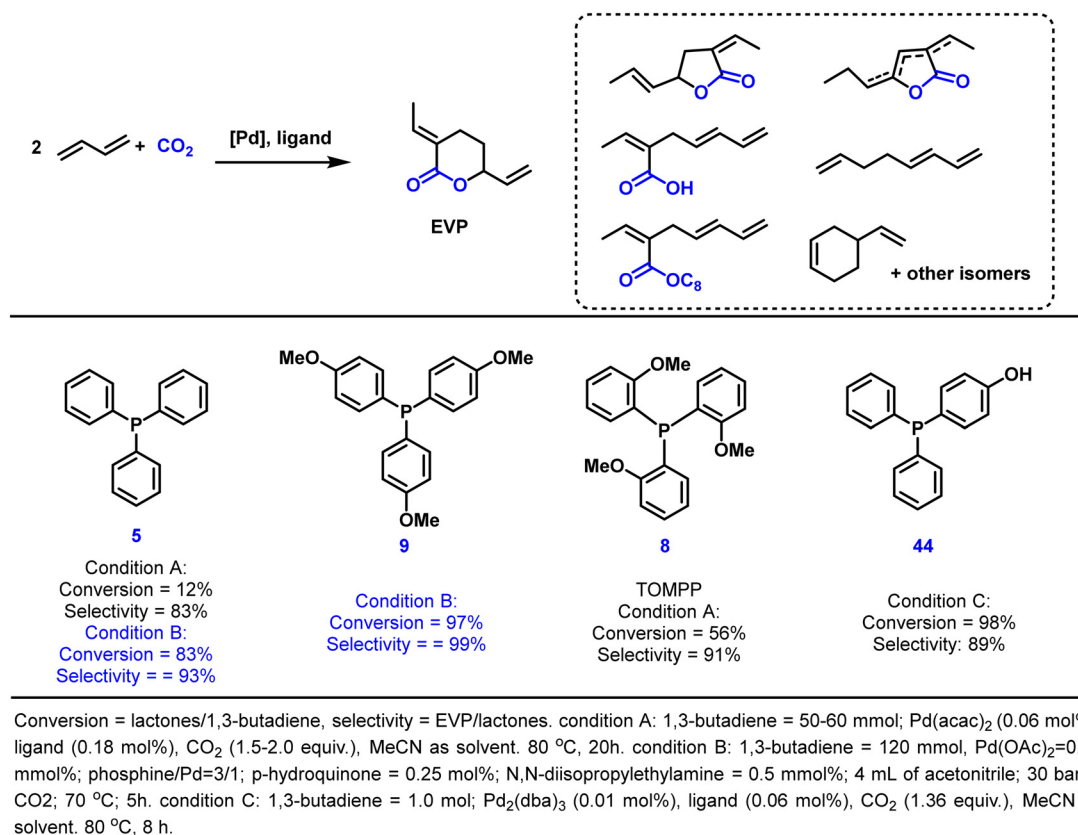
Scheme 3 Telomerization of 1,3-butadiene with CO 2 and representative catalytic systems.
