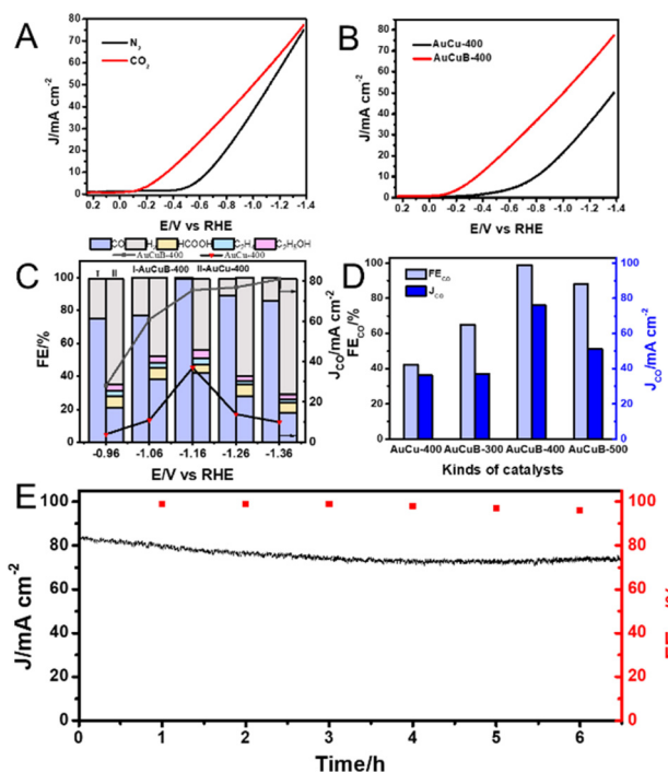
Fig. 2 (A) LSV curves recorded at a scan rate of 50 mV s −1 in 1 M KOH for AuCuB-400. (B) LSV curves recorded at a scan rate of 50 mV s −1 for AuCu-400 (black line) and AuCuB-400 (red line) in 1 M KOH under a CO 2 atmosphere. (C) FE and J CO measured at various potentials for the AuCu-400 and AuCuB-400 catalysts. (D) FE CO and J CO on AuCu-400, AuCuB-300, AuCuB-400, and AuCuB-500 at −1.16 V vs. RHE. (E) Long-term electrolysis of AuCuB-400 at −1.16 V vs. RHE.
