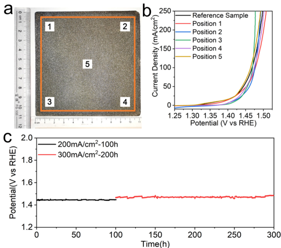
Fig. 6 Industrial application of the \text{Fe}^{\text{HV}}/\text{CeO}_2@\text{NF} electrode. (a) Photograph of the large-area ( 100 \text{ cm}^2 ) \text{Fe}^{\text{HV}}/\text{CeO}_2@\text{NF} electrode. (b) Polarization curves of the five different positions ( 1 \text{ cm}^2 ) in the large-area \text{Fe}^{\text{HV}}/\text{CeO}_2@\text{NF} electrode (the reference sample is directly synthesized with 1 \text{ cm}^2 ). (c) The chronopotentiometry measurements in 6 M KOH and at 60^\circ \text{C} .
