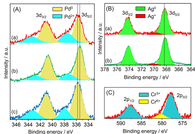
Fig. 2 (A) Pd 3d XPS spectra of (a) PdAgCr/amine-MSc, (b) PdAg/amine-MSc and (c) Pd/amine-MSc; (B) Ag 3d XPS spectra of (a) PdAgCr/amine-MSc and (b) PdAg/amine-MSc; and (C) Cr 2p XPS spectrum of PdAgCr/amine-MSc.
