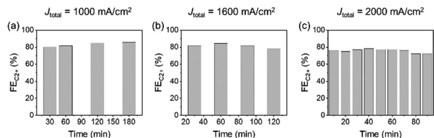
Fig. 5 FE_{C_{2+}} stability tests with respect to the current density over CuONPs-1.0/GDE in 1 M KCl under (a) J_{\text{total}} = 1000 \text{ mA cm}^{-2} , (b) 1600 \text{ mA cm}^{-2} and (c) 2000 \text{ mA cm}^{-2} .
