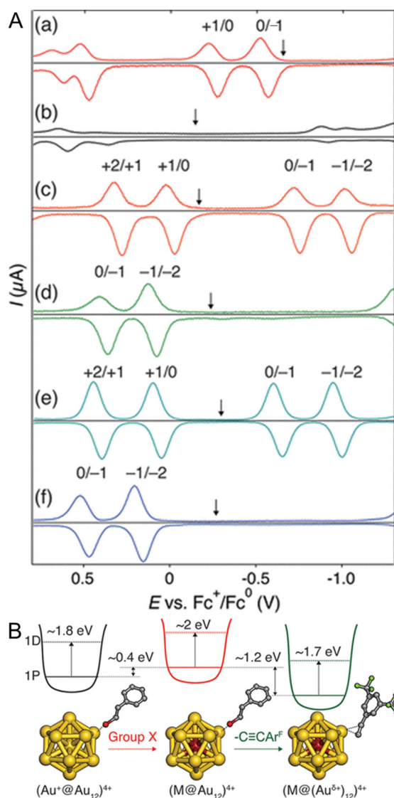
Fig. 8 (A) Differential pulse voltammograms of (a) [Au 25 (PET) 18 ] − , (b) [Au 25 (C≡CAr F ) 18 ] − , (c) [PtAu 24 (PET) 18 ] 0 , (d) [PtAu 24 (C≡CAr F ) 18 ] 2− , (e) [PtAu 24 (PET) 18 ] 0 , and (f) [PtAu 24 (C≡CAr F ) 18 ] 2− in a CH 2 Cl 2 solution of 0.1 M TBAPF 6 at room temperature. The down arrows indicate the corresponding open-circuit potentials. (B) Schematic energy diagram of M@Au 12 superatoms protected by thiolate or alkynyl groups. Reproduced with permission from ref. 104. Copyright 2019, American Chemical Society.
