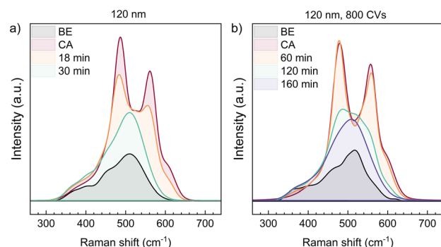
Fig. 2 Overlapped in situ Raman spectra of NiOOH reduction for two 120 nm NiO samples in 1 M KOH: a) before conditioning, in b) the sample was conditioned by 800 CVs to form more \text{Ni}(\text{OH})_2 . At 1.50 V vs. RHE (labelled “CA”), vibrations of NiOOH at 480\text{ cm}^{-1} and 560\text{ cm}^{-1} appear. The spectra are overlaid with spectra taken “x min” after stopping chronoamperometry. They show the gradual transformation of the spectral line back to the one characteristic for NiO before electrochemistry (labelled “BE”).
