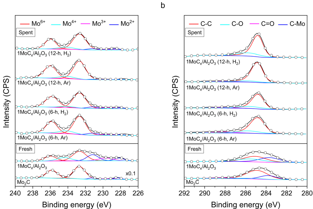
Fig. 6 XPS spectra of fresh and spent MoC x catalysts for (a) Mo 3d and (b) C 1s.
