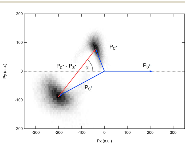
Fig. 4 Definition of the rotation angle \alpha measured between the momentum vector of the \text{S}^{2+} ion P_{\text{S}^{2+}} and the composite vector P_{\text{C}^+} - P_{\text{S}^+} .
