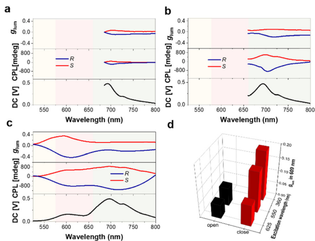
Fig. 4 (a–c) CPL spectra of R(S) -1-C-NR-Cy5 cholesteric texture ( \lambda_{\text{ex}} = 625 \text{ nm} , \lambda_{\text{ex}} = 550 \text{ nm} , \lambda_{\text{ex}} = 360 \text{ nm} , respectively). (d) 3D Column diagrams of CPL g_{\text{lum}} values obtained by irradiation of donor R -1 or acceptor dyes when CET was turned “on” and “off”, respectively.
