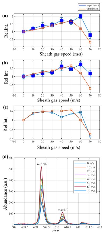
Fig. 3 (a) Relative intensity of the protonated reserpine ( m/z 609) and (b) the chemical noise at the sheath gas speed (0–70 m s -1 ). (c) The relative SNR of reserpine. (d) The mass spectra of reserpine at different sheath gas speeds.
