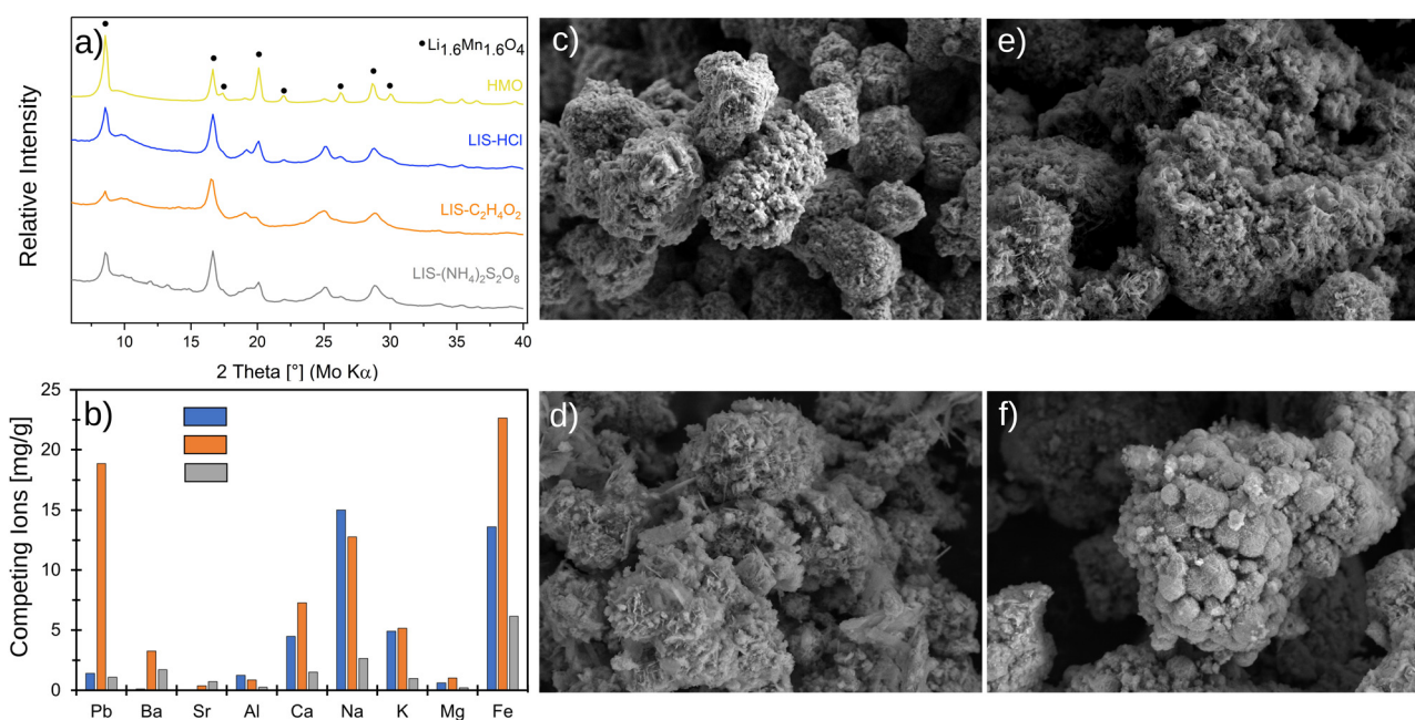
Fig. 2 (a) X-ray diffraction patterns of Mn-oxides, HMO indicates the raw adsorbent, LIS is the lithium-ion-Sieve treated with various desorption agents over eight cycles. (b) Accumulation of various cations originating from geothermal brine. SEM images of (c) raw adsorbent ( \text{H}_{1.6}\text{Mn}_{1.6}\text{O}_4 ) and with HCl (d), (\text{NH}_4)_2\text{S}_2\text{O}_8 (e) and \text{CH}_3\text{COOH} (f) treated adsorbent after eight cycles.
