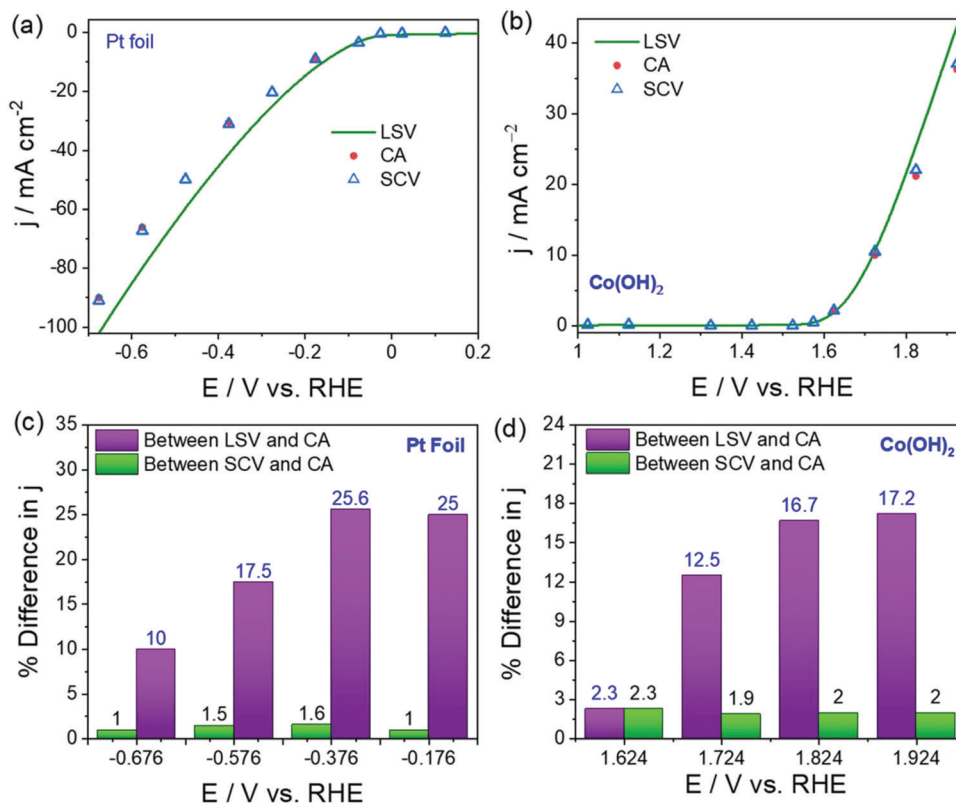
Fig. 4 (a) HER polarization curves of Pt foil acquired using LSV and SCV and provided in comparison with CA data. (b) OER polarization curves of Co(OH) 2 acquired using LSV and SCV and provided in comparison with CA data. (c and d) The plots of % difference in j between LSV and CA, and SCV and CA against potential showing the closeness of SCV and CA. Reproduced from ref. 64 (Copyright 2022, IOP Publishing).
