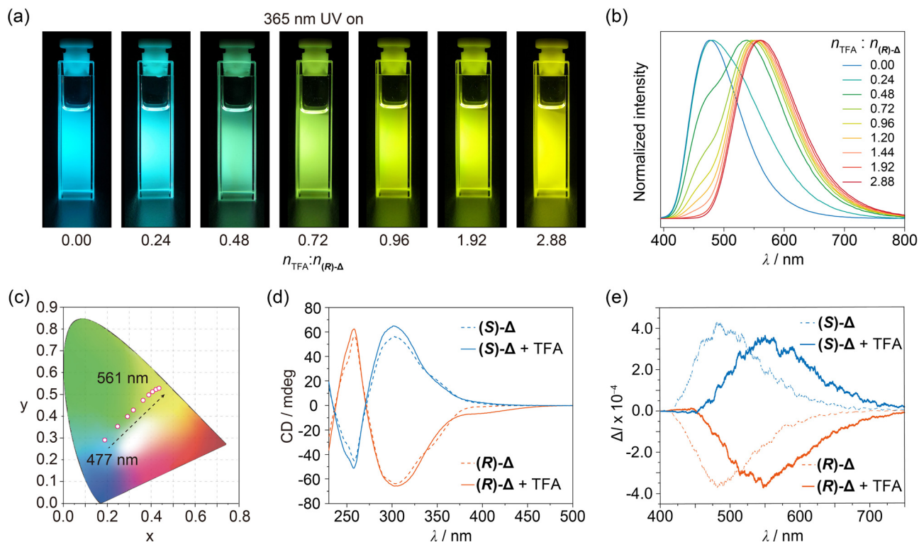
Fig. 3 Photophysical properties of ( R )- and ( S )- \Delta . (a) Luminescence photographs taken upon shining 365 nm UV light. (b) Fluorescence spectra upon excitation at 380 nm. (c) Trajectory of tuning colors shown in the CIE coordinate diagram of solutions ( 1 \times 10^{-5} M) of ( R )- \Delta in \text{CHCl}_3 containing different amounts of TFA relative to ( R )- \Delta ranging from 0 to 2.88 equiv. (d) CD and (e) CPL spectra of solutions ( 2 \times 10^{-4} M) of ( R )- and ( S )- \Delta in deacidified \text{CHCl}_3 (dash line) and in acidified \text{CHCl}_3 with TFA ( 2.88 \times 10^{-5} M, solid line).
