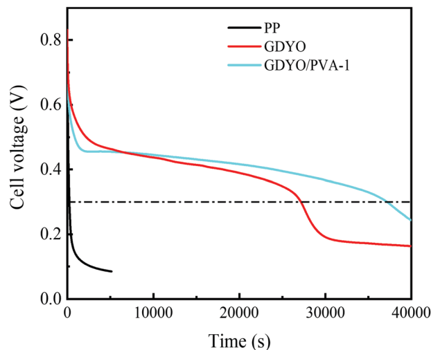
Fig. 5 SDC of the supercapacitors with different membranes when the electrolyte is a 1 M H 2 SO 4 and 0.5 M KI mixture.
