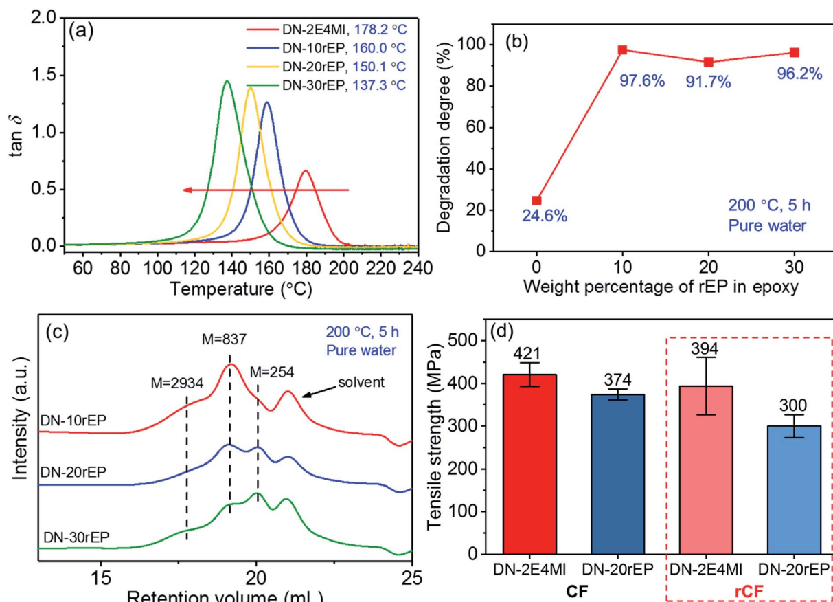
Fig. 5 (a) \tan \delta of the cured epoxies that use the rEP to replace part of the DER epoxy resin. The tests were performed at a heating rate of 3 \text{ K min}^{-1} ; (b) effects of rEP content in the cured epoxy on the degradation degree; (c) GPC curves of the decomposed polymer of DN-10rEP, -20rEP and -30rEP; (d) tensile strengths of DN-2E4MI and DN-20rEP with 3 layers of CF and rCF.
