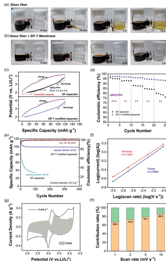
Fig. 3 Optical images of an H-type electrolytic cell with an aqueous solution of 1 M LiI and 0.1 M I 2 in the left chamber and a 0.5 M Li 2 SO 4 aqueous solution using a GF separator (a) and a ZIF-7 modified separator (b). (c) Electrochemical aging test (from 0.5 to 3 hours resting after fully charging) for half cells with the AC working electrodes using a GF separator (upper) and a ZIF-7 modified separator (lower) at 0.5 A g -1 . (d) CE of the cells with a GF separator and a ZIF-7 modified separator at different aging durations. (e) Long-term cycling stability of the cells with a GF separator and a ZIF-7 modified separator. (f) Log( i ) versus log( v ) plots at specific peak currents. (g) CV curve with the calculated pseudocapacitive fraction shown by the shaded area at 2 mV s -1 . (h) Bar chart showing the percentage of the calculated pseudocapacitive contribution at 1.0–10.0 mV s -1 .
