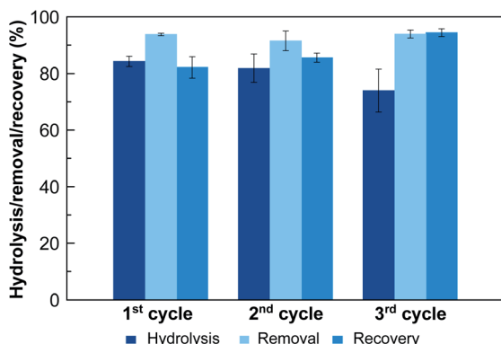
Fig. 4 Recyclability studies of MOF-808_60 along three successive cycles: (i) simultaneous hydrolysis of methyl paraoxon and removal of phosphate and (ii) subsequent recovery of phosphate by exchange with hydrogencarbonate anions. After each cycle, MOF-808_60 was regenerated by treatment with an aqueous solution of hydrochloric acid (2.5 mM).
