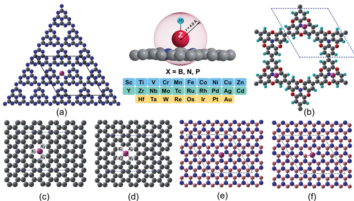
Fig. 1 Proposed 2D materials with TM embedded at various defect sites. (a) g-C_3N_4 (b) 2DCP (c) graphene with one C defect site (d) graphene with two C defects site (e) h-BN with one B defect site (f) h-B_2N_2 with one B and one N defects site. The labeled sites ( x_1-x_4 ) in light gray color in (c) and (d) represent the non-metal (B, N, P) doping sites in single and dual type doping fashion. Color code: metal, magenta; B, light pink; N, blue; C, gray; O, red; H, cyan.
