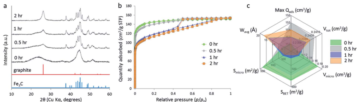
Fig. 9 (a) XRD data, (b) N 2 adsorption/desorption isotherms and (c) porimetry data for carbons prepared by pyrolyzing starch and Fe(NO 3 ) 3 to 800 °C for various hold-times. Figure reproduced with permission from ref. 108.
