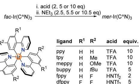
Scheme 2 Chemically induced fac → mer isomerizations are possible for different Ir(C ^ N) 3 complexes using either TFA or HNTf 2 for the protonation step.
