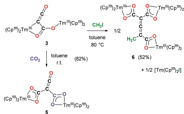
Scheme 2 Reactivity of 3 towards \text{CO}_2 and \text{MeI} .
