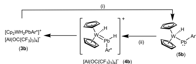
Scheme 8 (i): + Me NHC, toluene/o-DFB, rt, 3 h, – [ Me NHC–H][Al(OC{CF 3 }) 4 ]. (ii): + [H(Et 2 O) 2 ][Al(OC{CF 3 }) 4 ], toluene/C 6 H 4 F 2 , rt, – 2 Et 2 O.
