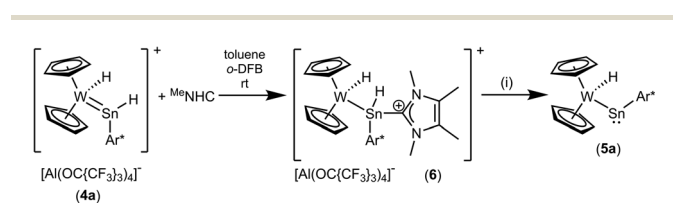
Scheme 5 (i): Toluene/o-DFB, 80 °C, 3d, – [ Me NHC–H][Al(OC{CF 3 }) 4 ].
