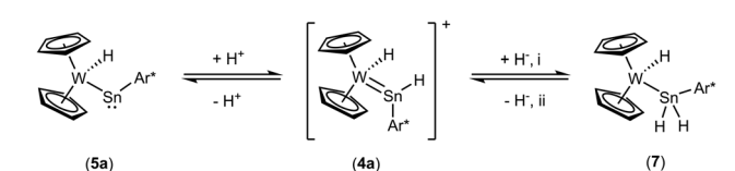
Scheme 6 Addition and abstraction of protons and hydride ligands. (i): rt, LiAlH 4 , Et 2 O; (ii): rt, [Ph 3 C][Al(OC{CF 3 }) 4 ], o-DFB.
