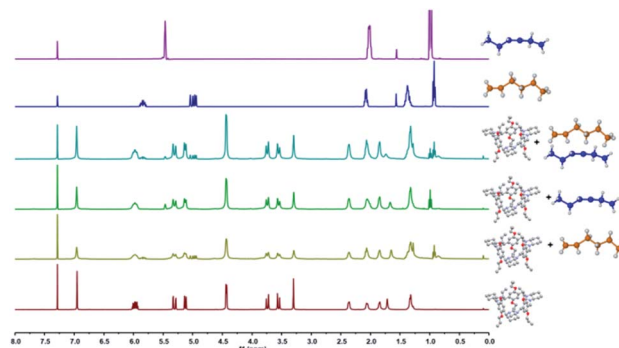
Fig. 2 1 H NMR spectra (400 MHz, chloroform-d, 298 K) of activated P-TA, activated P-TA after adsorption of vapor 1-He, activated P-TA after adsorption of vapor trans-3-He, activated P-TA after adsorption of the vapor 1-He/trans-3-He mixture for 16 h, 1-He and trans-3-He. The solid samples were dried after vapor adsorption and then dissolved in chloroform-d for analysis.
