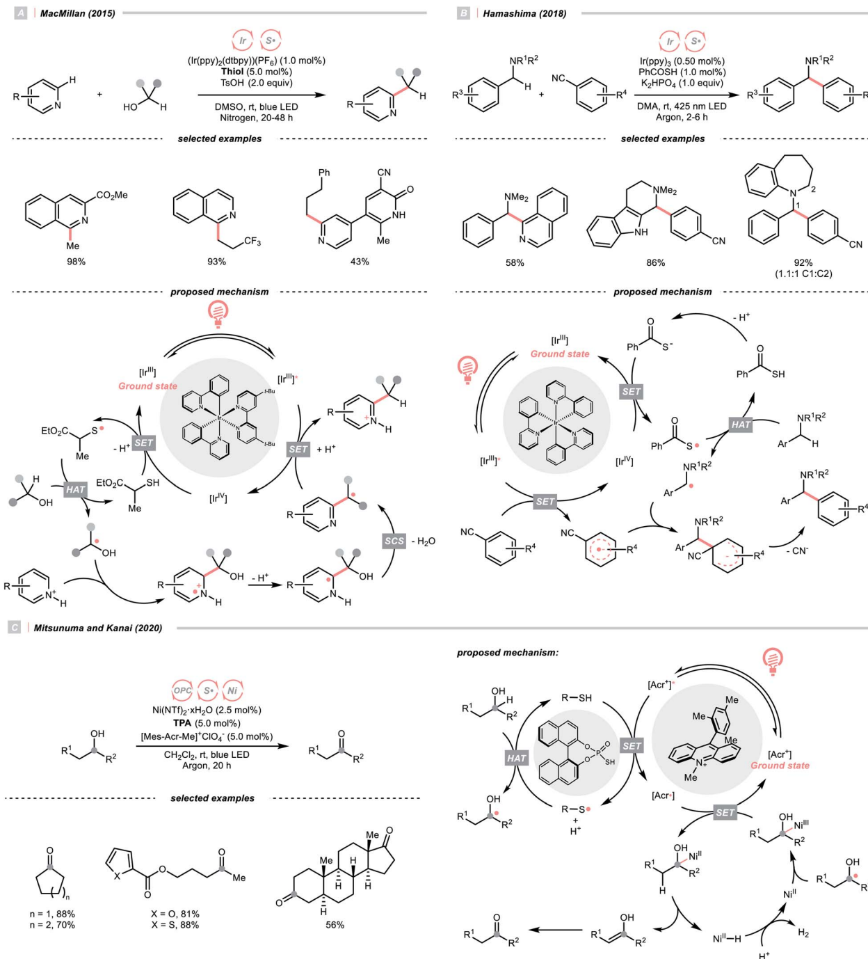
Scheme 16 Thiol radical-enabled \text{C}(\text{sp}^3)\text{-H} elaborations.
