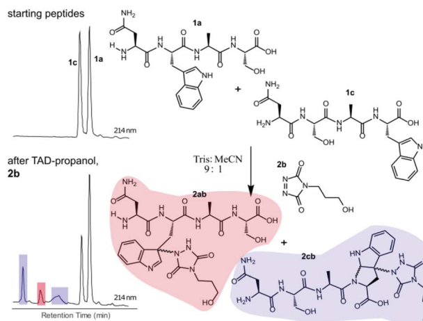
Fig. 2 Competition experiment of NWAS ( 1a , 0.3 mM) and NSAW ( 1c , 0.3 mM) peptides with TAD-propanol ( 2b , 0.5 mM) in Tris buffer pH 5.8. Zoom of the HPLC chromatogram at 214 nm of the starting mixture (top left) and after reaction with TAD-propanol 2b (bottom left). Based on peak integration of the starting peptide XIC chromatograms before and after conjugation 25% of 1c was converted while around 8% of 1a was converted.
