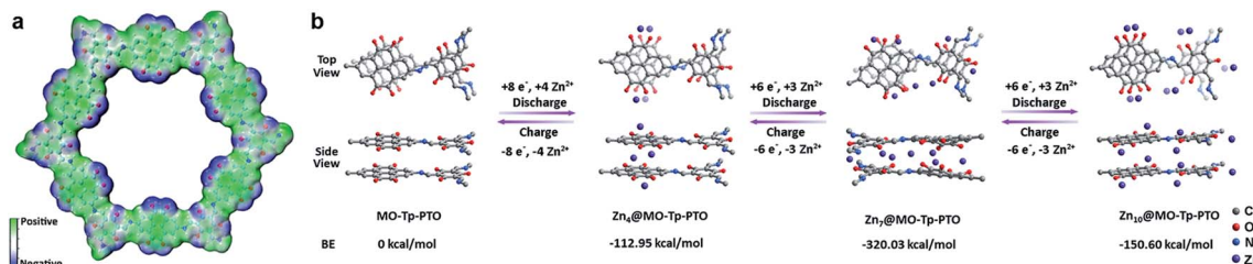
Fig. 5 (a) Electronegativity simulation of Tp-PTO-COF; (b) simulation of binding energies with different numbers of Zn 2+ ions in MO-Tp-PTO.
