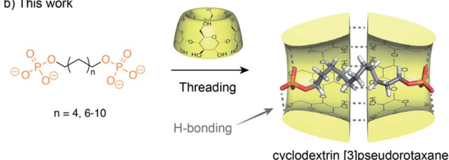
Fig. 1 (a) Previous work on compression of alkyl chains by self-assembled capsules or boxes. (b) Alkyl diphosphate axles used in this study and corresponding CD [3]pseudorotaxane with potential compression resulting from hydrogen bonding and hydrophobic interactions between the threaded axle and head to head CDs.
