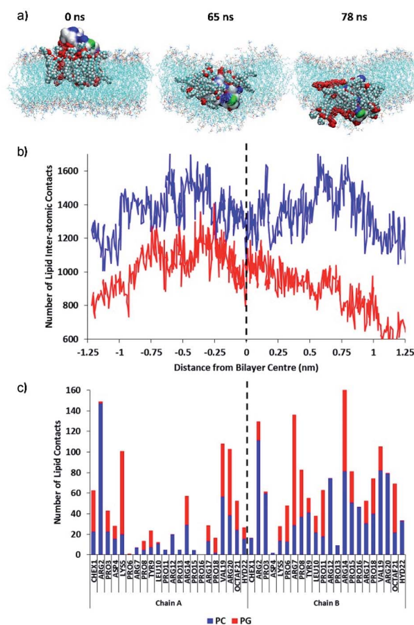
Fig. 12 (a) MD simulation snapshots of the permeation of octo-fluorobiphenyl dimer-NH 2 7 into the model membrane. The PrAMP is shown as a surface and colour-coded according to residue charge (blue = Arg, green = neutral polar, white = non-polar). The annular lipids are also shown as large spheres, with PG in red. (b) Total number of contacts between the PrAMP with PC (blue line) and PG lipids (red line) with respect to approximate position of the peptide centre-of-mass relative to the bilayer centre (dotted black line). (c) Average numbers of contacts between each PrAMP residue with PC (blue) and PG (red) for each of the two AMP chains in the octo-fluorobiphenyl-dimer during membrane permeation.
