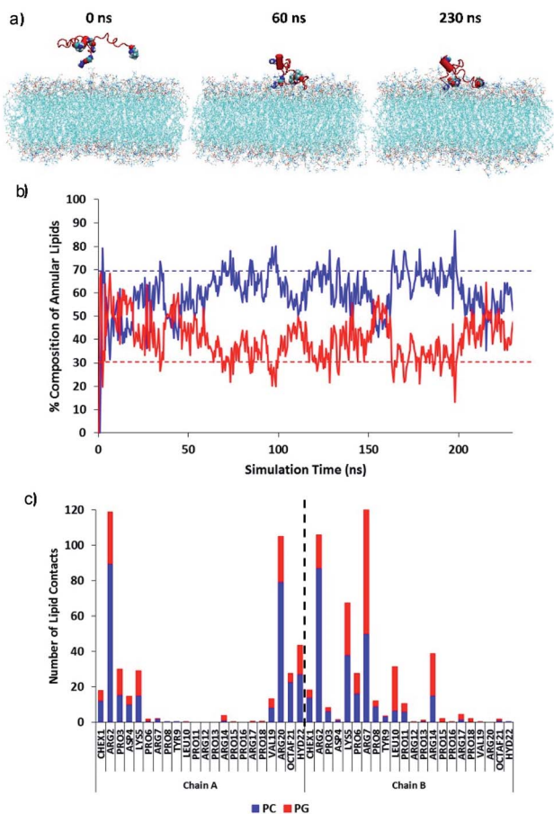
Fig. 11 (a) MD simulation snapshots of the initial adsorption of octo-fluorobiphenyl dimer-NH 2 7 to the model membrane. The PrAMP backbone is shown as a red ribbon. Chex, hydrazide (–NHNH 2 ) and octo-fluorobiphenyl groups are shown as large spheres. (b) Time series plots of the compositions of PC (blue line) and PG lipids (red line) whose atoms lie within 0.4 nm of the PrAMP. Nominal bulk percentages for PC (70%) and PG (30%) are shown as dotted lines. (c) Average numbers of contacts between each PrAMP residue with PC (blue) and PG (red) for each of the two PrAMP chains of the octo-fluorobiphenyl dimer-NH 2 7.
