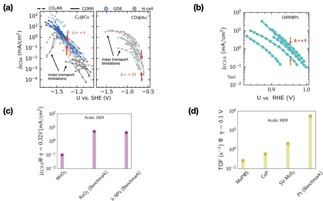
Fig. 3 (a) ECSA normalized current density ( j_{\text{ECSA}} ) for \text{CO}_2 and \text{CO} reduction ( \text{CO}_2\text{RR} ) to \text{C}_2 products and \text{CO}_2\text{RR} to \text{CO} on various nanostructured/modified Cu 35–50 and Au electrodes, 51–59 respectively. The data include experiments performed in GDEs and H-cells, (b) ECSA normalized current density for the ORR on nanostructured/Pt alloys. 60–66 \Delta represents the variation in ECSA normalized activity in the kinetically controlled regions. Regions limited by mass transport are highlighted by arrows. (c) ECSA normalized current density at an overpotential ( \eta ) of 0.32 V for \text{MnO}_2 electrodes (based on earth-abundant Mn) compared to the benchmark Ir/Ru based electrodes for the OER in acid 67–69 (d) TOF at an overpotential ( \eta ) of 0.1 V for the HER in acid on several non-precious metal electrodes compared to the benchmark Pt. 28,70–72
