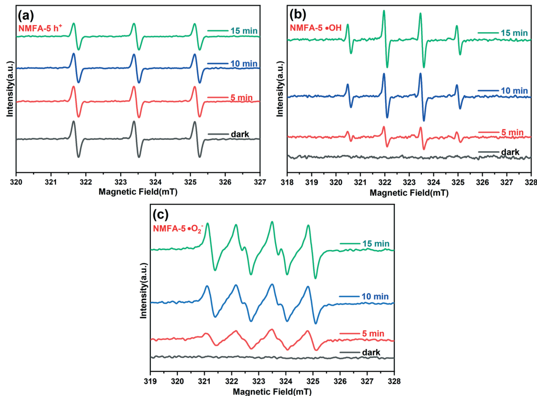
Fig. 14 The ESR spectra of (a) h^+ , (b) \cdot\text{OH} and (c) \cdot\text{O}_2^- generated using the NMFA-5 composites.
