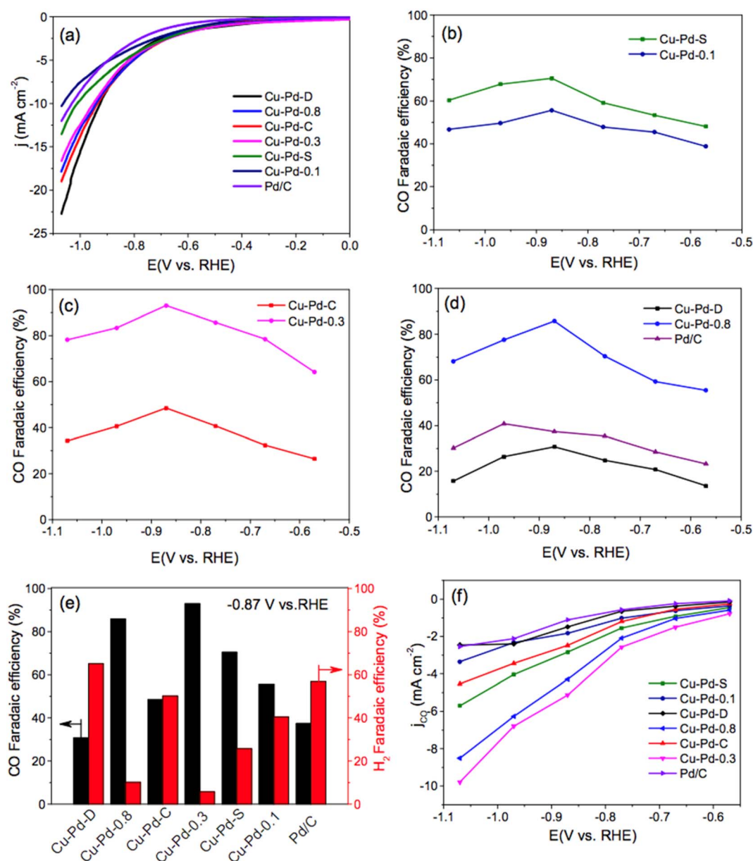
Fig. 8 LSV curves (a) of bimetallic Cu–Pd–S, Cu–Pd–0.1, Cu–Pd–C, Cu–Pd–0.3, Cu–Pd–D, Cu–Pd–0.8 nanoalloys, commercial Pd/C catalyst in \text{CO}_2 saturated 0.5\text{ M KHCO}_3 solution with a scan sweep of 10\text{ mV s}^{-1} , the CO faradaic efficiency at different applied potentials (b–d), the CO and \text{H}_2 faradaic efficiency at a fixed potential of -0.87\text{ V} (e), and CO partial current density of these nanoalloys (f). Reproduced with permission. 91 Copyright ©2018, American Chemical Society.
