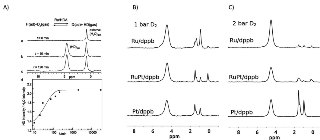
Fig. 13 (A) Upper panel: Gas phase 11.4 Tesla 1 H NMR spectra showing the production of HD from the reaction of Ru/hexadecylamine nanoparticles containing adsorbed H with gaseous D 2 in a glass sealed NMR tube (for details see Pery et al. 184 ). (B and C) Typical 1 H gas-phase NMR spectra after exposing solid MNPs at room temperature to 1 bar or 2 bar D 2 gas for 16 h with Ru/dppb, RuPt/dppb and Pt/dppb nanoparticles at two different pressures of D 2 gas. The chemical shift of the HD signal is set to 4.5 ppm (for details see Rothermel et al. 185 ).
