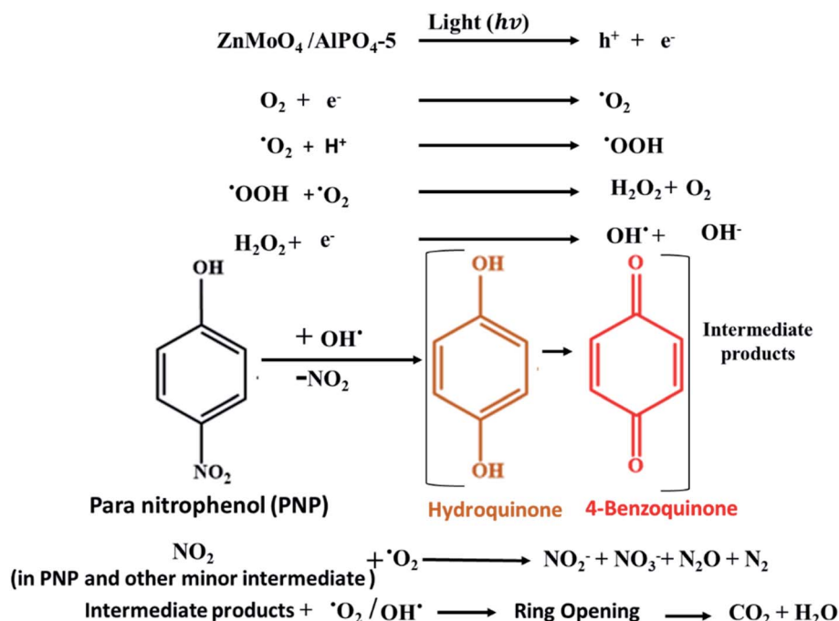
Scheme 1 The proposed mechanism of the photocatalytic degradation of PNP on \text{ZnMoO}_4 / \text{AlPO}_4-5 catalysts.
