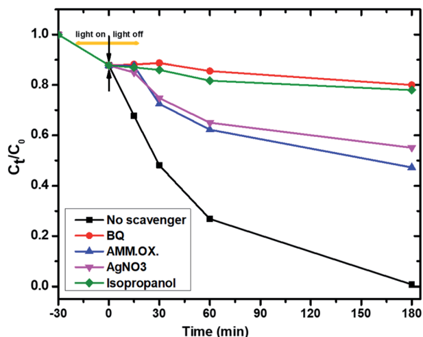
Fig. 12 Inhibition of the photocatalytic degradation of PNP with different active-species scavengers BQ (for \cdot\text{O}_2^- ), IPA (for \cdot\text{OH} ), AO (for \text{h}^+ ) and \text{AgNO}_3 (for \text{e}^- ). Reaction conditions: the dosage of catalyst 1.0 \text{ g l}^{-1} , initial PNP concentration of 0.04 \text{ g l}^{-1} after 180 min irradiation time.
