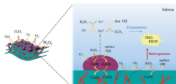
Fig. 12 Possible reaction mechanism of \text{CoNWs}@/\text{CoAl-LDHs}/\text{Fe}_3\text{O}_4 .
