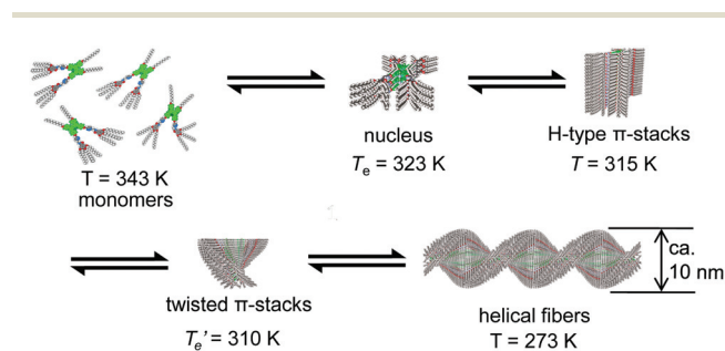
Fig. 3 Schematic assembly mechanism for the formation of helical fibrous aggregates Agg. II L of dye 1 upon slow cooling from 343 K to 273 K in the chiral limonene solvent.
