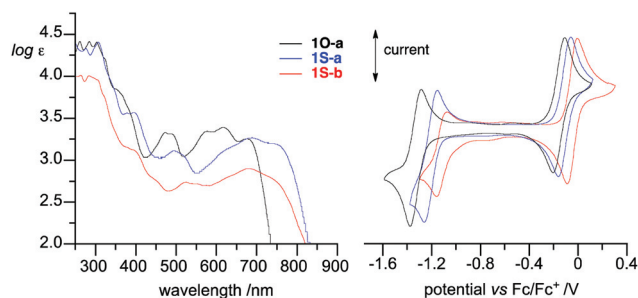
Fig. 5 Left: UV/vis spectra in \text{CH}_2\text{Cl}_2 and right: Cyclic voltammograms (0.5 mM in \text{CH}_2\text{Cl}_2 [ n\text{-Bu}_4\text{N}^+\text{PF}_6^- ] (50 mM), at \sim 20^\circ\text{C} , 50 \text{mV s}^{-1} , glassy carbon working electrode) for radicals 1O-a (black), 1S-a (blue), and 1S-b (red).
