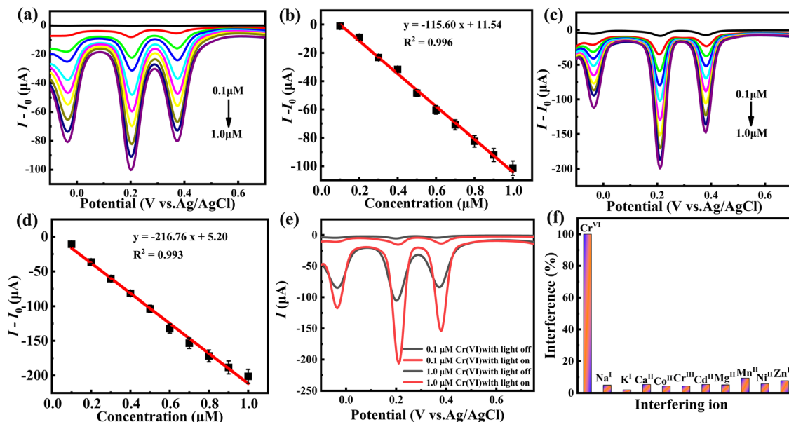
Fig. 4 (a) DPV curves of hybrid 1 modified electrodes in 0.5 M H 2 SO 4 with continuous addition of Cr(VI) under dark conditions; (b) The corresponding linear dependences; (c) DPV curves of 1 in 0.5 M H 2 SO 4 with successive changes in concentrations of 0.1 and 1.0 μM Cr(VI) under visible light illumination; (d) The linear dependence curve of 1 ; (e) Control experiments showing DPV curves of 1 with continuous addition of Cr(VI) under dark or light illumination; (f) Current interference of 1 towards Cr(VI) with different interferents of 40 μM Na + , K + , Ca 2+ , Co 2+ , Cd 2+ , Cr 3+ , Mg 2+ , Mn 2+ , Ni 2+ , and Zn 2+ to mix with 4 μM Cr(VI), respectively.
