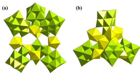
Fig. 28 Views of (a) [(\text{Nb}_4\text{O}_{12})(\text{H}_2\text{O})_3]\text{Nb}_4\text{O}_{12}(\text{H}_2\text{O})_3\text{O}_{13}\text{H}_8(\text{H}_2\text{O})_4]^{24-} and (b) [(\text{Nb}_7\text{O}_{22}\text{H}_2)_4(\text{UO}_2)_7(\text{H}_2\text{O})_6]^{22-} . Color codes are the same as in Fig. 1; Nb, lime.
