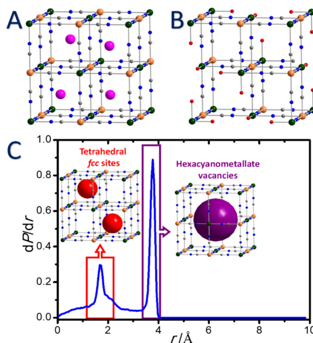
Fig. 1 Crystalline structure of non-lacunar (A) and lacunar (B) PBA, \text{A}_{1-x}\text{M}'[\text{M}'(\text{CN})_6]_{1-x/3}\cdot n\text{H}_2\text{O} . Colour code: orange, M'; green, M; magenta, A'; blue, N; grey, C. The oxygen of \text{H}_2\text{O} coordinated to the \text{M}^{n+} ions are represented by red spheres; (C) pore size distribution of PBA obtained from Monte Carlo simulations illustrating the presence of two types of pores corresponding to the tetrahedral sites of the fcc structure and the larger pores formed by hexacyanometallate vacancies.
