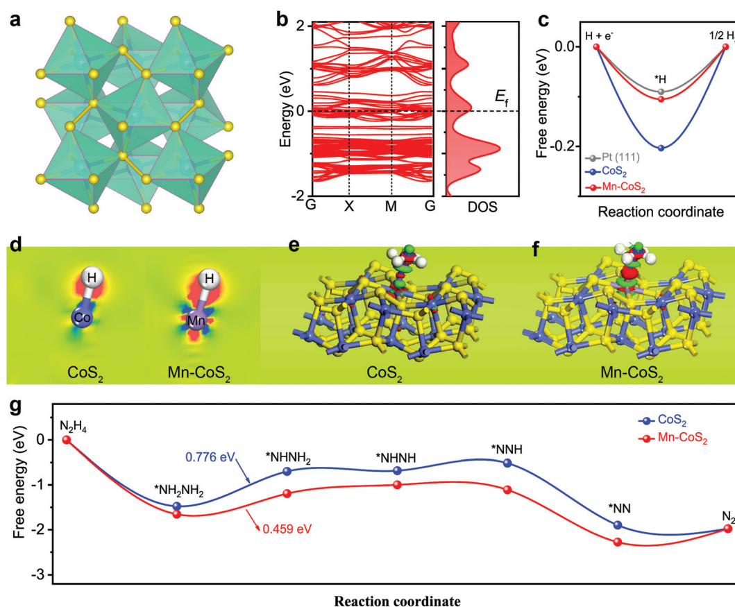
Fig. 1 DFT calculation results: (a) crystal structure of \text{CoS}_2 ; (b) the calculated electronic band structure and the corresponding DOS results of \text{Mn-CoS}_2 ; (c) the free energy profiles of HER pathways for \text{CoS}_2 and \text{Mn-CoS}_2 ; (d) the charge density difference contour plot of Co–H and Mn–H regions, the red and blue colors represent the accumulation and depletion of electrons, respectively; (e and f) the side-view of the three-dimensional charge density difference of the H-adsorbed configuration at different sites over the catalyst surface, the pink and green region representing charge depletion and accumulation in the space, respectively; (g) the free energy profiles of the HzOR reaction pathways for \text{CoS}_2 and \text{Mn-CoS}_2 .
