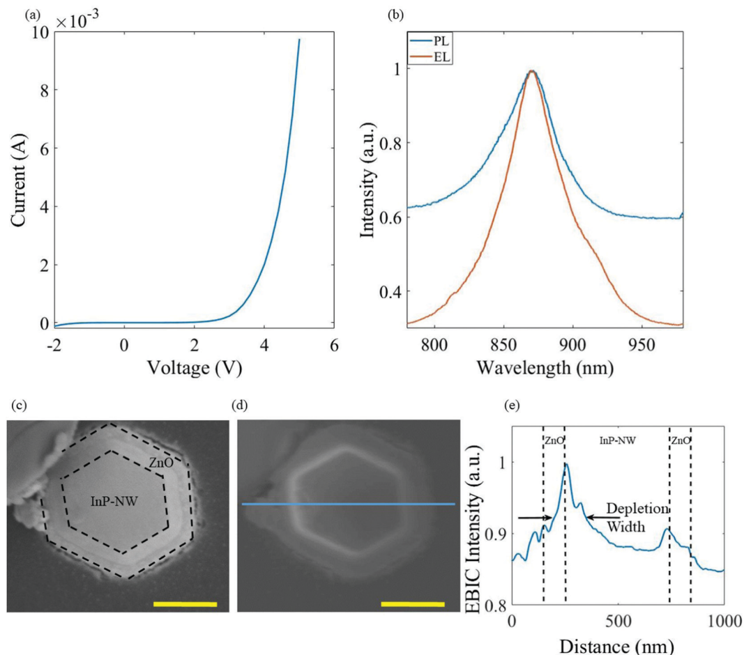
Fig. 2 (a) I - V characteristics of the on-substrate device at room temperature. (b) PL spectrum at a 17 \mu\text{W} excitation power and EL spectrum at a 5 \text{ mA} current. (c) SEM image of a single NW from the fabricated LED array. The image on the top left corner is the contact probe in good contact with the ZnO shell. (d) EBIC signal acquired under an accelerating voltage of 10 \text{ kV} corresponding to the SEM image in (c). (e) EBIC scan profile across the NW, indicated by the blue solid line. Scale bars in (c) and (d) are 300 \text{ nm} .
