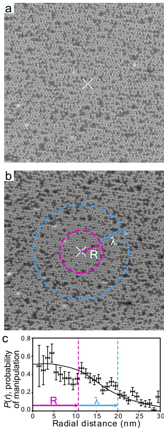
Fig. 1 Nonlocal molecular manipulation induced by charge injection from an STM tip. (a) and (b) 50 \text{ nm} \times 50 \text{ nm} images ( +1 \text{ V} , 100 \text{ pA} ) of \text{Si}(111)-7 \times 7 partially covered with toluene molecules (dark-spots) before (a) and after (b) hole injection ( -1.4 \text{ V} , 250 \text{ pA} , 20 \text{ s} ) into the white \times . (c) Probability of nonlocal manipulation (see main text for definition) of toluene molecules adsorbed to unfaulted-middle (UM) sites as a function of radial distance from the injection site (white \times ) for -1.5 \text{ V} , 900 \text{ pA} , 45 \text{ s} injection. Black line is a fit to a two-step ballistic-diffusive transport model 22,31 with ballistic length scale R = (12.8 \pm 1.5) \text{ nm} and diffusive length scale \lambda = (11.0 \pm 0.3) \text{ nm} also marked as circles in (b).
