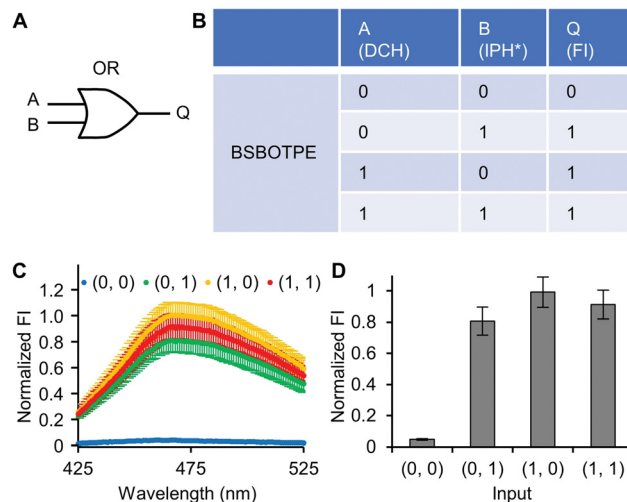
Fig. 4 OR logic operation. (A) Symbol of logic gate. (B) Truth table. (C) The normalized fluorescence spectra of logic operation with different inputs. (D) Normalized FI at 471 nm. The concentrations of DCH (or IPH*) and BSBOTPE used are 6 \mu\text{M} and 141 \mu\text{M} , respectively. Excitation wavelength was set at 350 nm. n = 3 .
