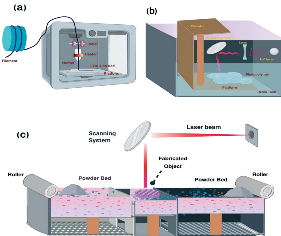
Fig. 2 Schematic representation of AM fabrication processes: (a) fused deposition modeling, (b) stereolithography and (c) selective laser melting 48 (created with BioRender).
