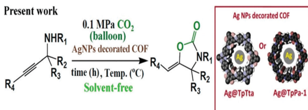
Scheme 37 The synthesis of 2-oxazolidinones using an AgNP-decorated COF. Reproduced with permission from ref. 56; copyright: 2020, ACS Sustainable Chemistry & Engineering.
