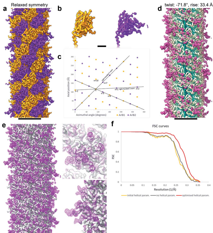
Fig. 3 Refining helical parameters after symmetry relaxation. (a) CryoEM map of the M. villosus archaeallum filament solved with relaxed helical symmetry showing ArlB1 in orange and ArlB2 in purple. (b) Close-up of the head domains of ArlB1 (orange) and ArlB2 (purple). (c) Helical net diagram showing the positions of ArlB1 (orange dots) and ArlB2 (purple dots) in a two-dimensional plot. Solid black lines show various component helices. (d) CryoEM map of the archaeallum filament solved imposing helical symmetry with refined parameters of -71.8^\circ twist and 33.4 \text{ \AA} rise. The map is coloured in petrol blue–light yellow–magenta from the core to the periphery of the filament. (e) Superposition of the cryoEM map obtained relaxing the helical symmetry (solid grey) and cryoEM map obtained applying refined helical parameters (mesh magenta). Two close-ups show the peripheral areas best resolved using the refined helical parameters. (f) Fourier shell correlation curves comparison between the cryoEM maps obtained with initial helical parameters ( 108^\circ twist and 5.5 \text{ \AA} rise; orange), relaxed helical symmetry (grey), refined helical parameters ( -71.8^\circ twist and 33.4 \text{ \AA} rise; red). Scale bar in (a, d, e), 50 \text{ \AA} ; in (b), 10 \text{ \AA} .
