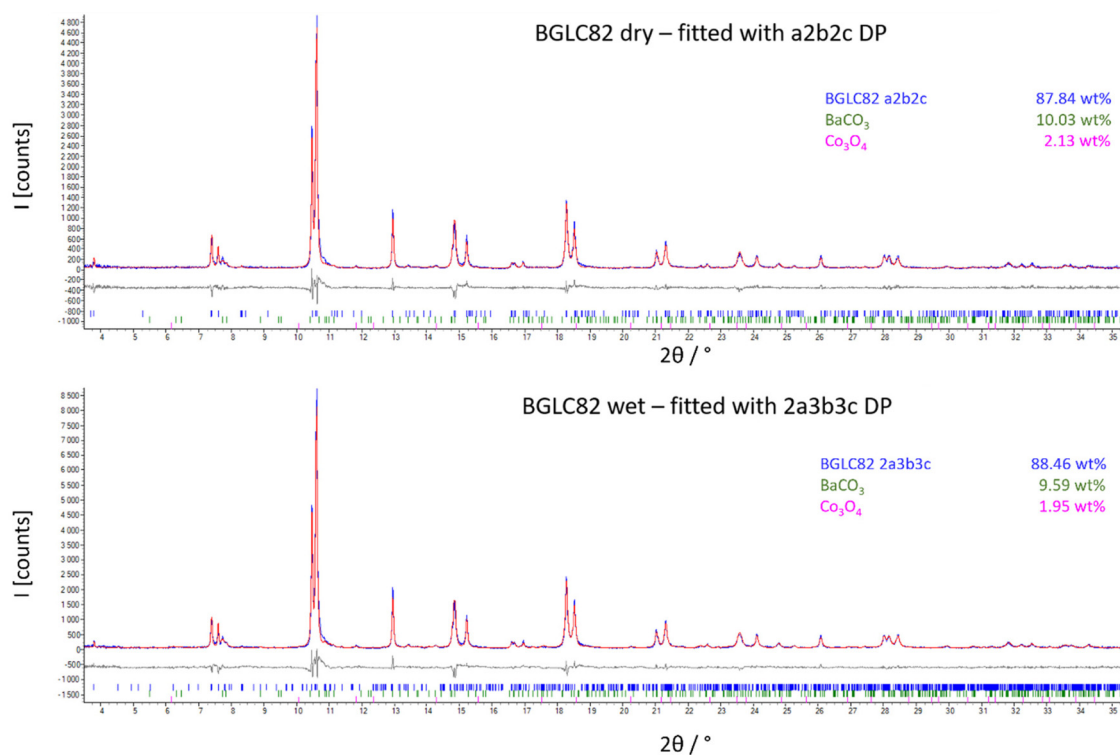
Fig. 8 SR-PXD of BGLC82 treated in dry (upper) and wet (lower) atmosphere at 300 °C. The spectra are fitted to a Pm m a2b2c (dry), and a Pm m 2a3b3c (wet) unit cell.
